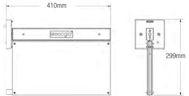
FLAG MOUNT
